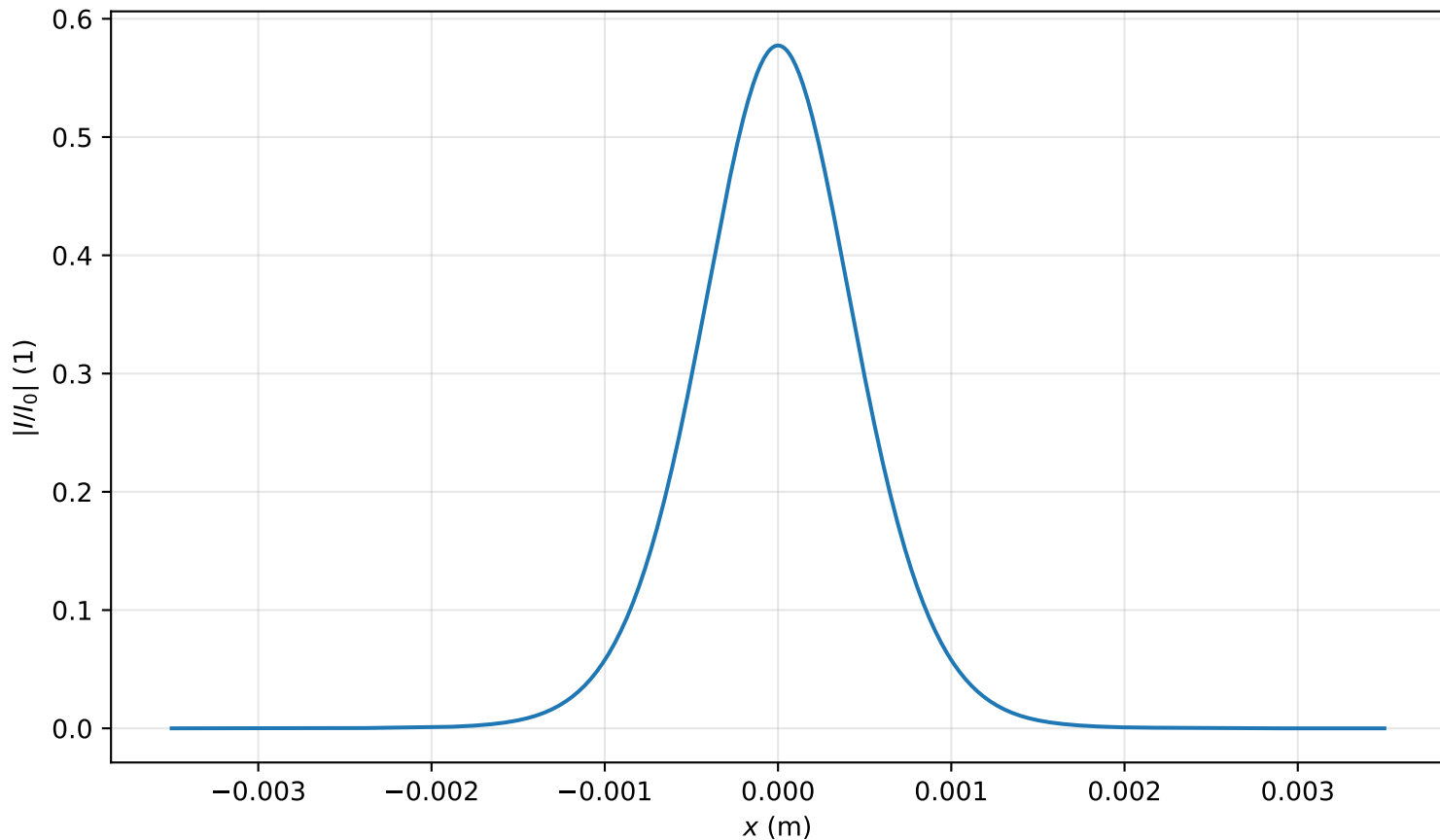
Intensity profile I(x, y = 0, z = 2.946m)/I_0 , P_{in}=0.5P_{cr} , artificial time
